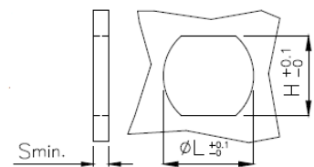
PANEL HOLE
